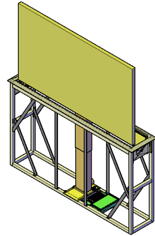
BKT-M595 Motorized TV Lifter (Flip Cover-Type2)
