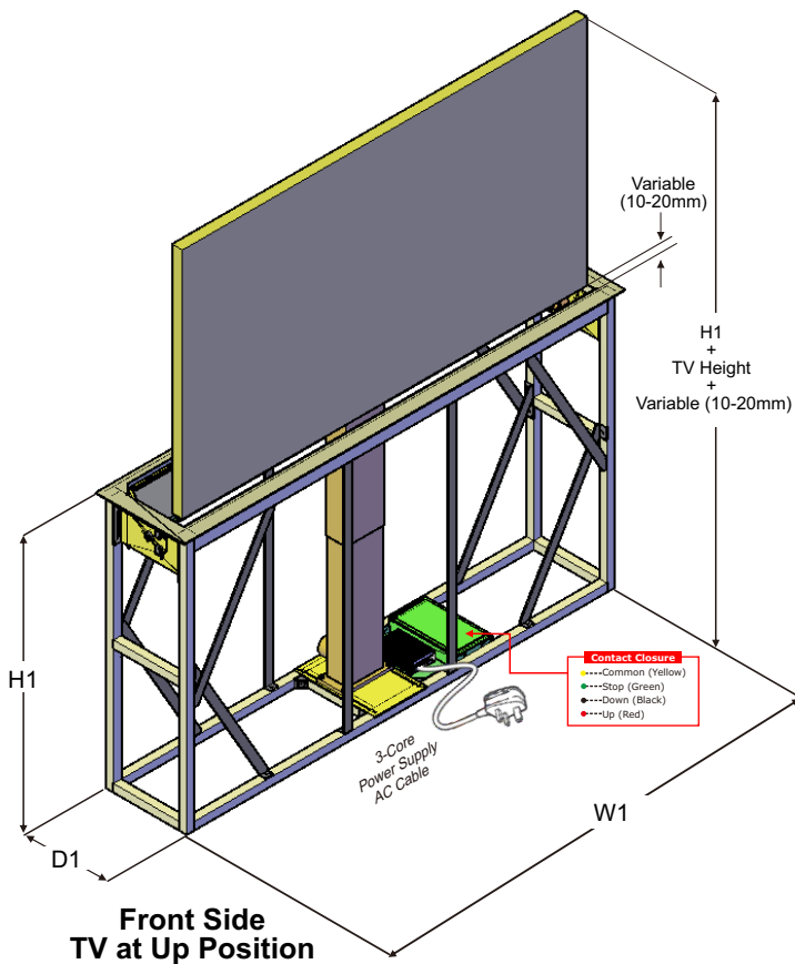
BKT-M595 Motorized TV Lifter (Top Cover-Type1)
